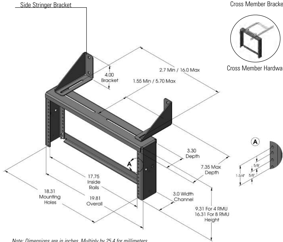
Cross Member Bracket
