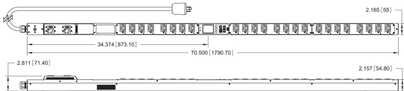
(P6-1F0A1 shown)
