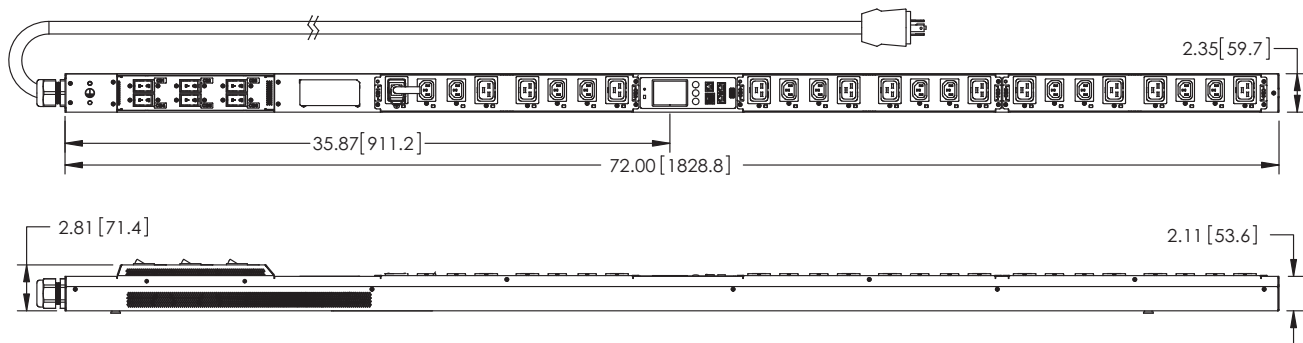
(P6-3U0M3 shown)
