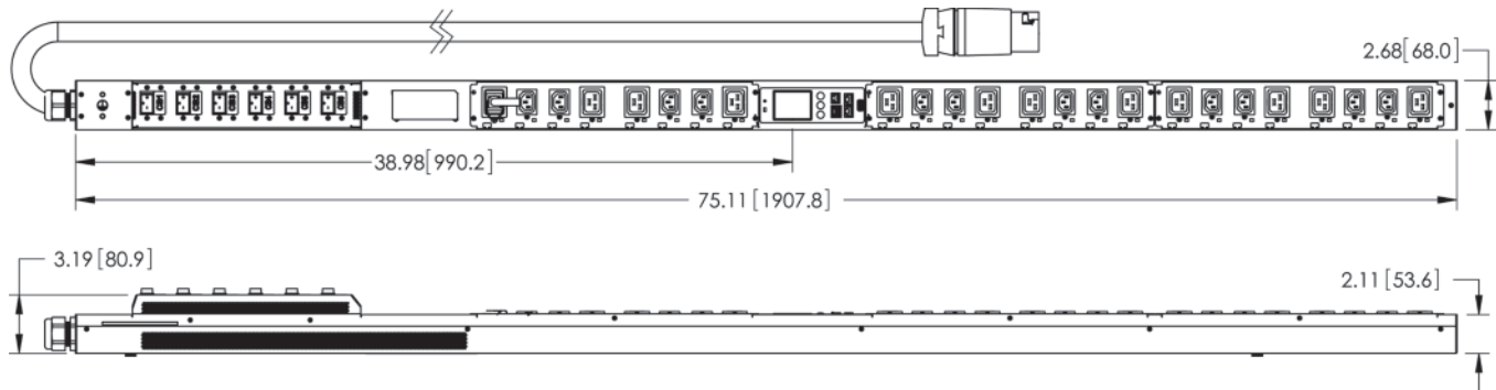
(P6-3U0M3 shown)
