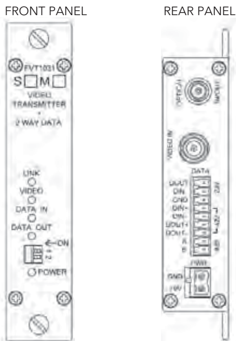
FIGURE 2 - FVT1031 TRANSMITTER
