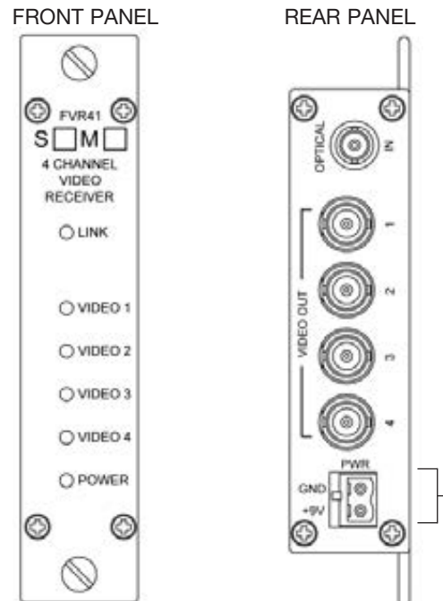
FIGURE 3 – FVR41 RECEIVER
