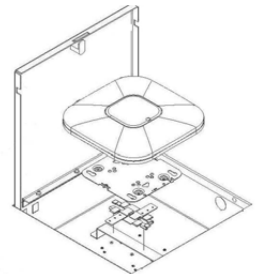
Figure 5 – Exploded door view.
