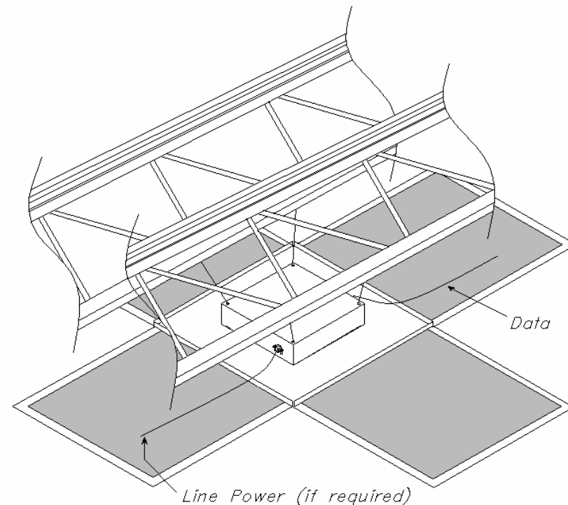
Figure 6 - Ceiling installation.
