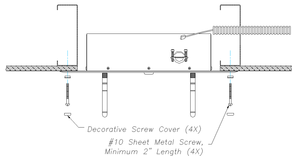
Figure 5 - Ceiling installation.
