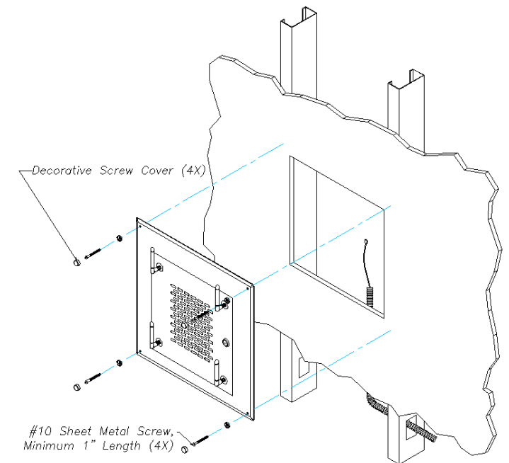
Figure 4 - Wall installation.
