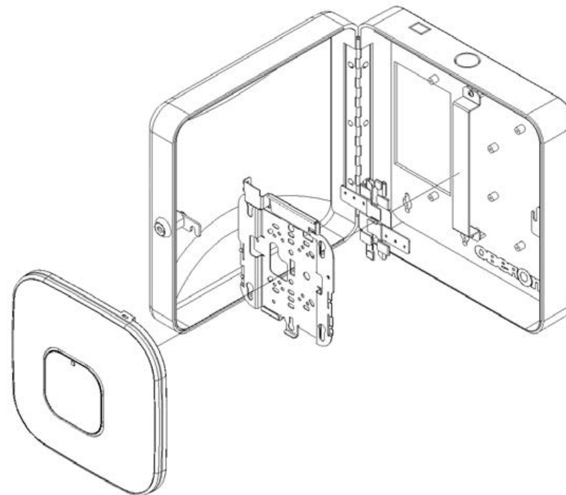
Figure 2 – Model 1015-00 Access Point Installation
