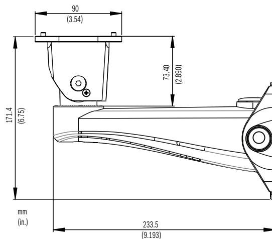
MBE-28B, side view
