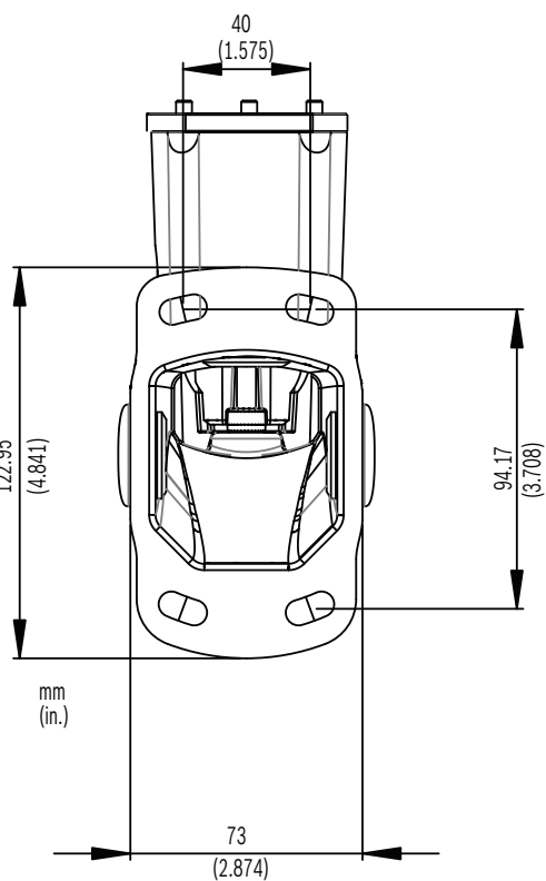
MBE-28B, rear view
