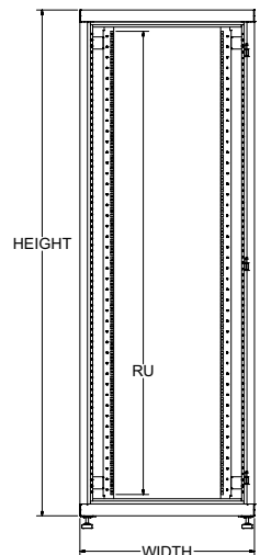
FRONT VIEW DOORS REMOVED FOR CLARITY
