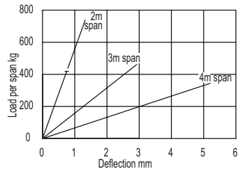
SPEEDWAY SW4 LOAD DEFLECTION DATA - CONTINUOUS BEAM
