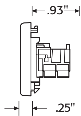
STANDARD FACEPLATE 2- or 4-Port (fits openings of approximately 1.38" x 2.70")
