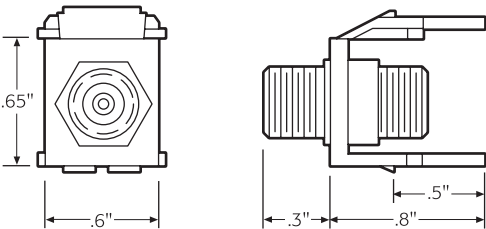
F-Type Connector
