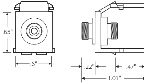
Simplex FC QuickPort Adapter
