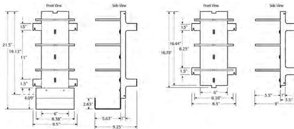
300 Pair Vertical Cord Manager for Extension Units
