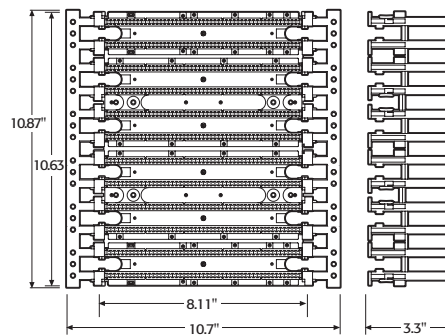
300 Pair Wiring Base (with legs)
