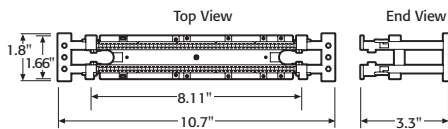
50 Pair Wiring Base (with legs)
