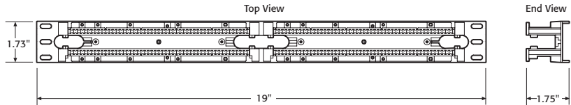
200 Pair Rack Mount Wiring Panel
