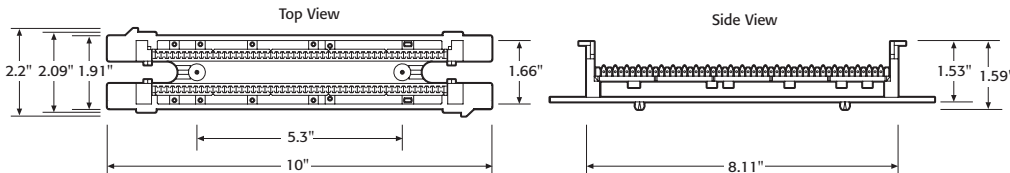
50 Pair 89D Bracket Compatible Wiring Base
