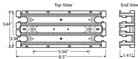
100 Pair Wiring Base (without legs)
