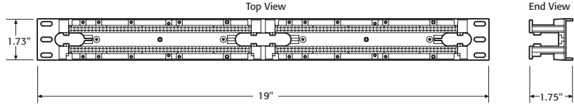
100 Pair Rack Mount Wiring Panel
