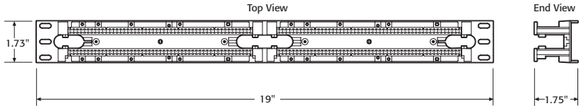
300 Pair Rack Mount Wiring Panel
