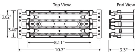
100 Pair Wiring Base (with legs)
