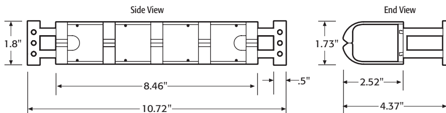
Horizontal Cord Manager with legs 41A10-HCM
