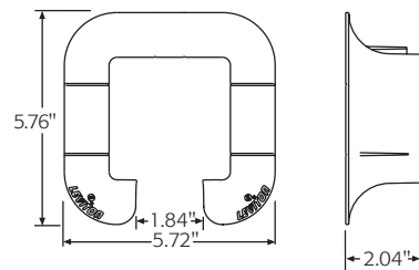
Bend-Radius Compliant Funnel (Use with 4x4 Vertical Slotted Duct only.)
