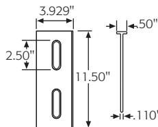
Vertical Channel Divider
