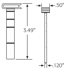
Cable Retainer
