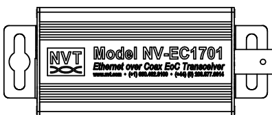
NV-EC1701 ETHERNET OVER COAX EoC TRANSCEIVER TOP VIEW
