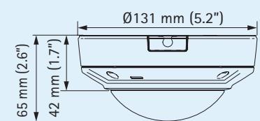
AXIS M3007-PV
