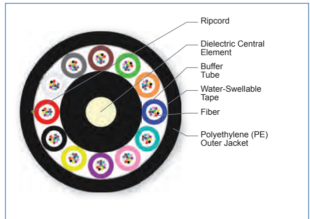
Cross Section of Part Number: 144EU4-T4101D20
