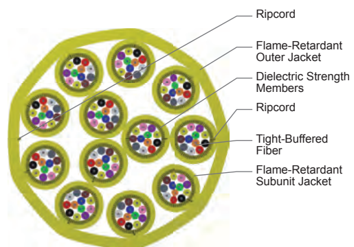
Cross Section of Part Number: 144E81-T3131-24
