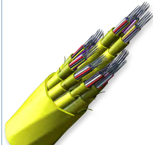
Part Number: 144E81-T3131-24
