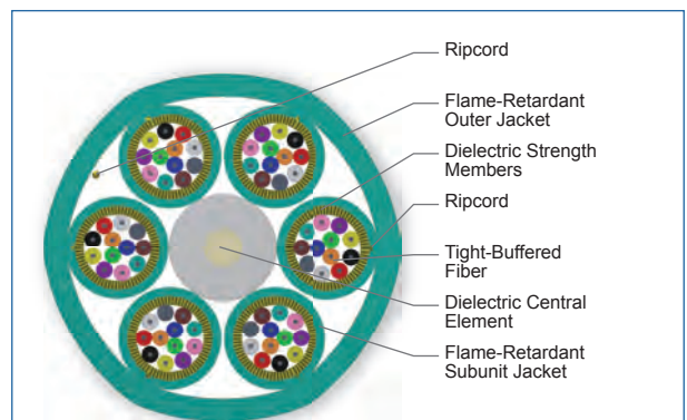
Cross Section of Part Number: 072T81-T3180-24
