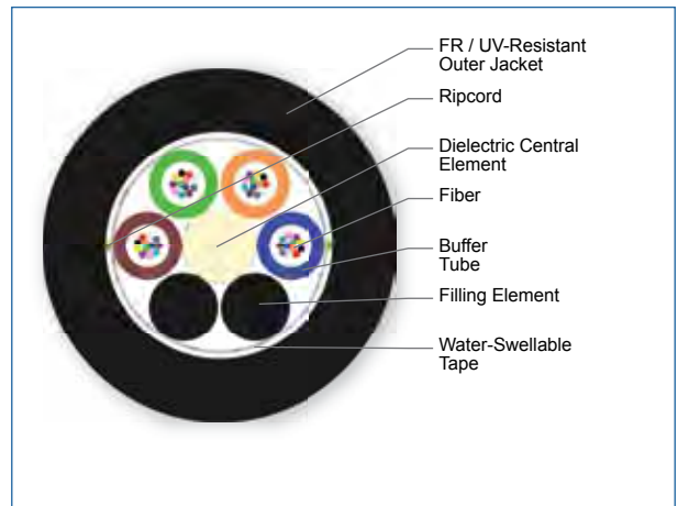
Cross Section of Part Number: 048TUF-T4180D20
