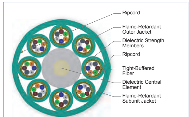
Cross Section of Part Number: 048T88-61190-29
