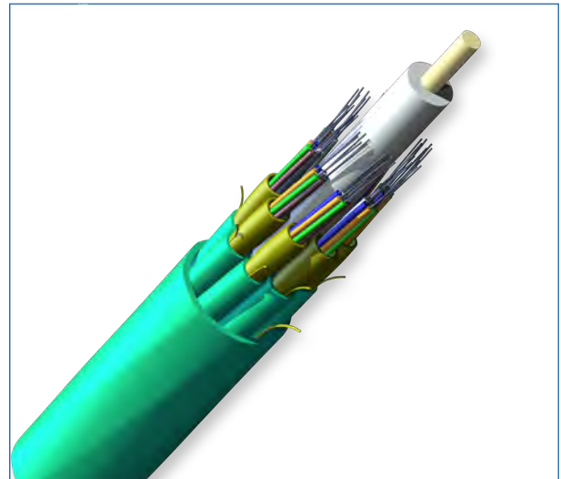
Part Number: 048T88-61190-29
