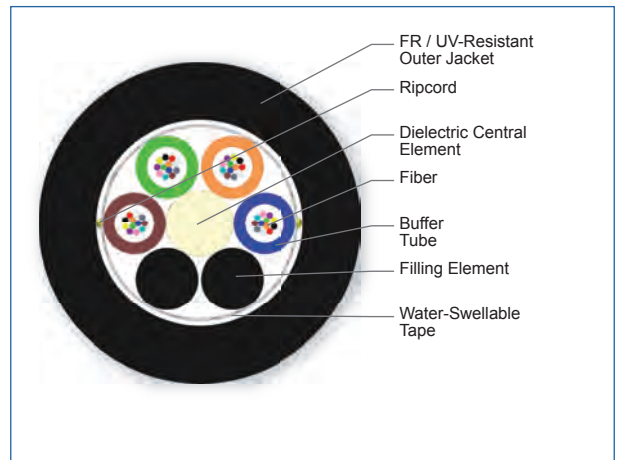
Cross Section of Part Number: 048KUF-T4130D20
