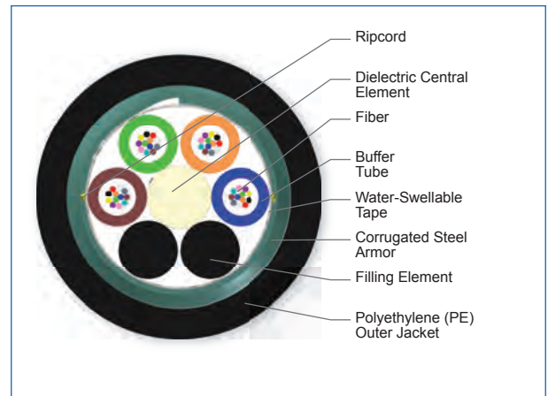
Cross Section of Part Number: 048KUC-T4130D20
