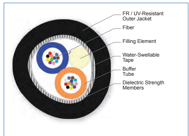
Cross Section of Part Number: 024TSF-T4131D20
