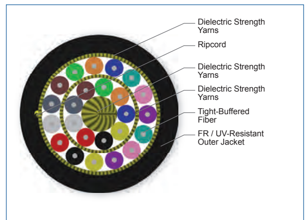
Cross Section of Part Number: 024T8P-31131-29
