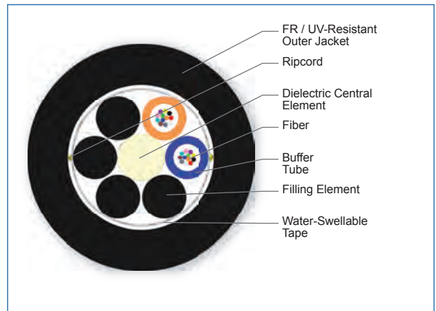
Cross Section of Part Number: 024KUF-T4130D20
