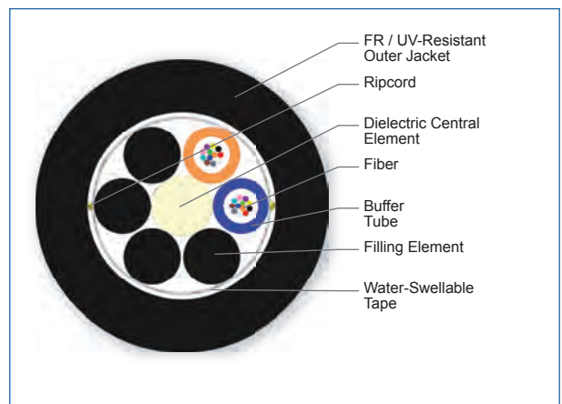
Cross Section of Part Number: 024EUF-T4101D20
