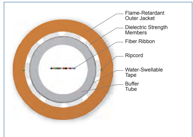
Cross Section of Part Number: 012TC8-14131-20
