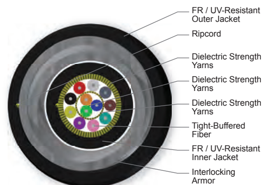
Cross Section of Part Number: 012K8P-31130-A3
