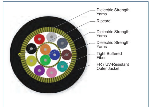
Cross Section of Part Number: 012E8P-31131-29
