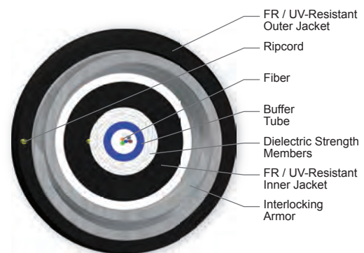
Cross Section of Part Number: 006TSF-T4180DA1
