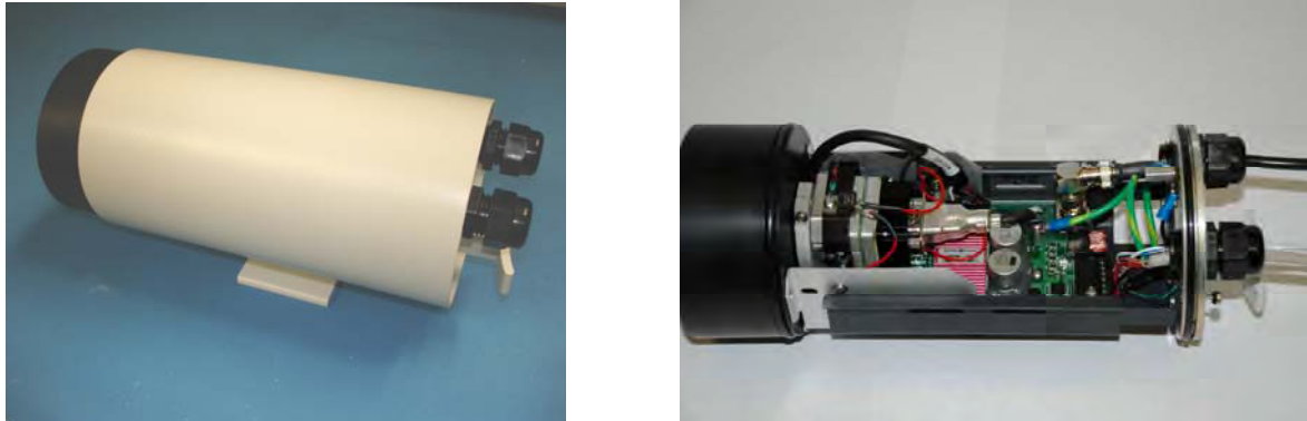
Figure 2-3: SR-309 Camera with and without the Environmental Enclosure
