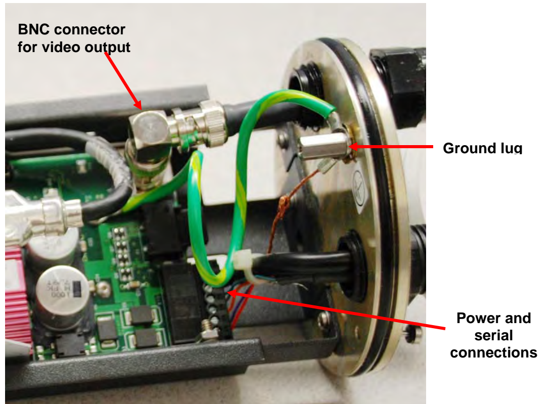
Figure 4-3: SR-Series Connections
