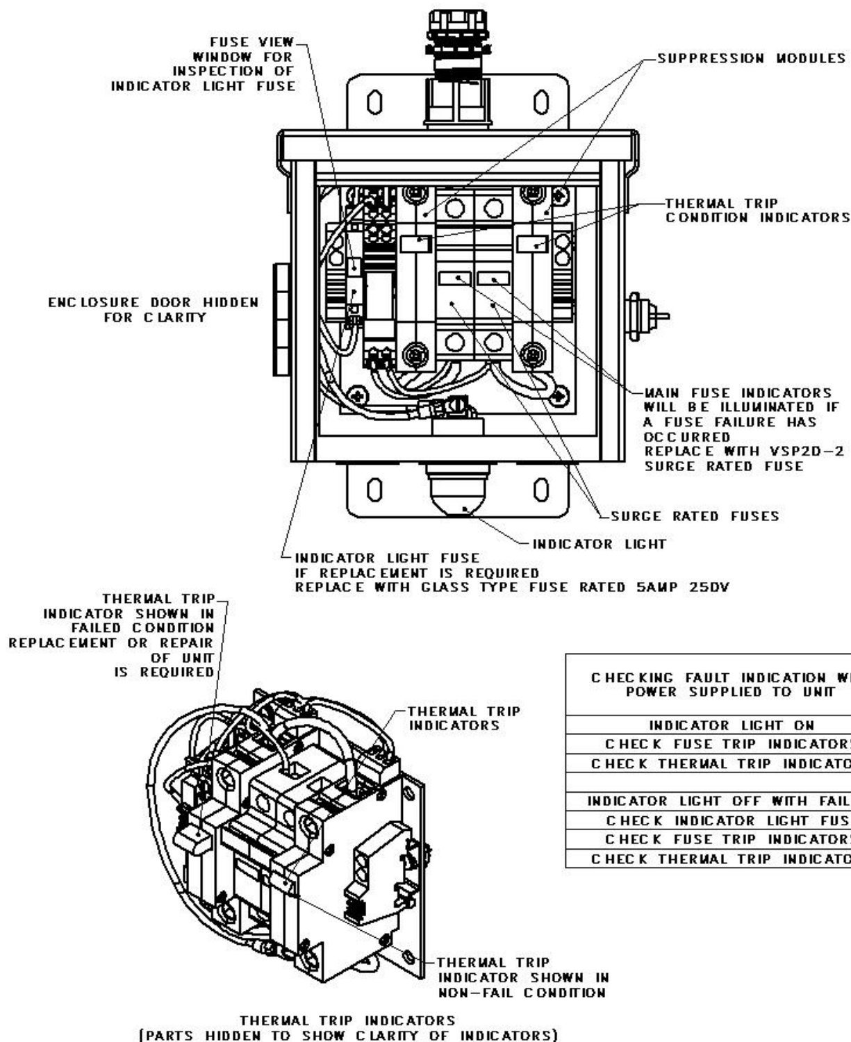
Fig 3. Fuse/Thermal location & Trip Indicators
