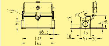
Blind way for one cable entry
