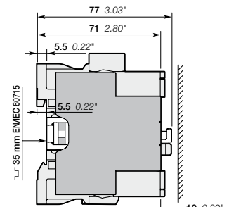
NF22E + CAL4-11 2-pole auxiliary contact block
