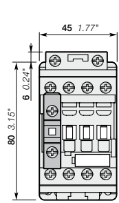
NF22E + CA4, CC4 1-pole auxiliary contact block
