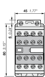
NF22E + CA4 4-pole auxiliary contact block
