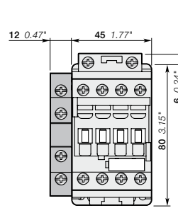
NF22E + CAL4-11 2-pole auxiliary contact block
