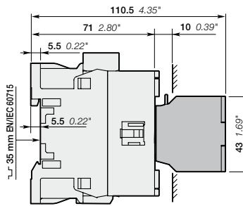
NF22E + CA4 4-pole auxiliary contact block
