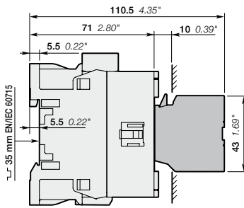
NF22E + CA4, CC4 1-pole auxiliary contact block
