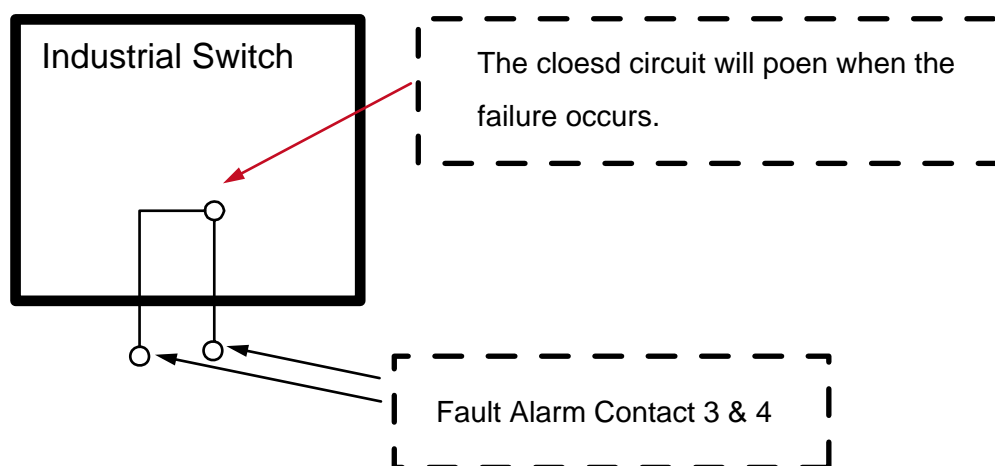
Figure 6: Alarm schematic
