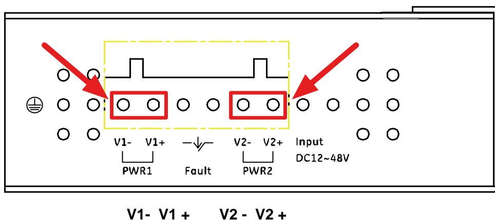
Figure 3: Power Inputs
