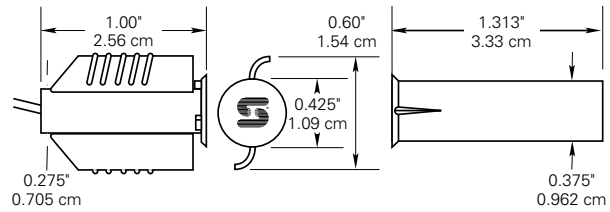
* Note: Wings compress to .375" dia. Magnet Part No. 1924 (Included)
