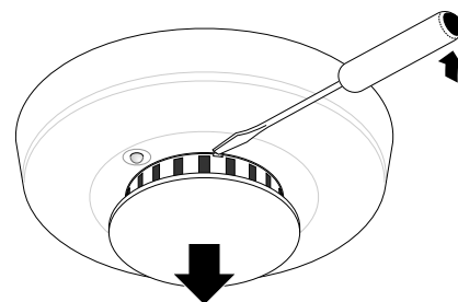
Figure 9. Removing the detector cap
