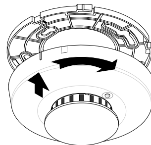
Figure 4. Mounting
