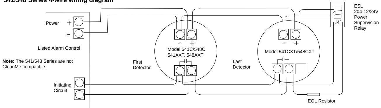
Figure 6. Wiring diagrams
