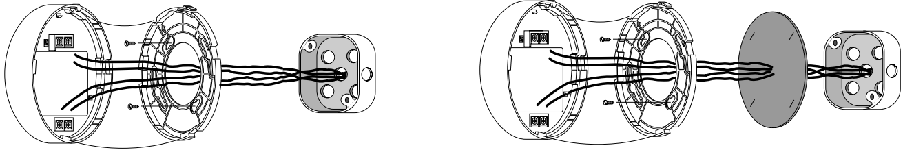
Figure 5. Detector installation
