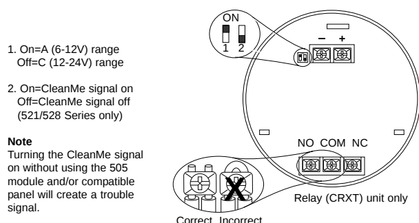
Figure 1. Switches
