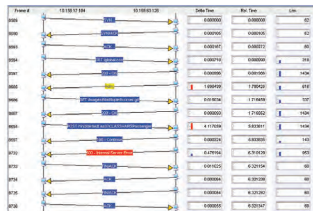
Powerful bounce charts visualize application turns
