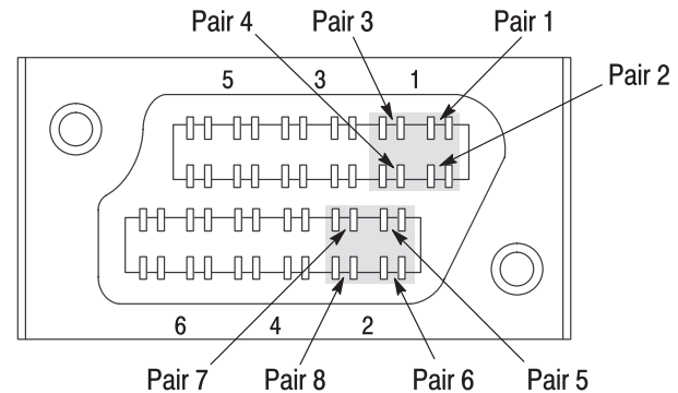
MRJ21 Receptacle (Back of Patch Panel)
