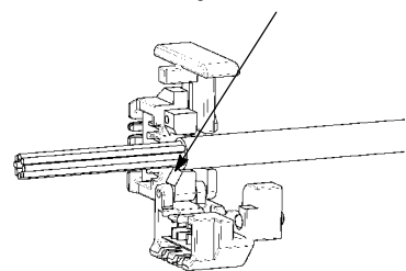
Align Cable Jacket With Shelf
