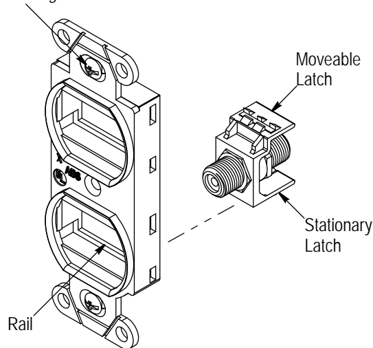
Tighten Duplex Strap to Electrical Box Using Mounting Screws
