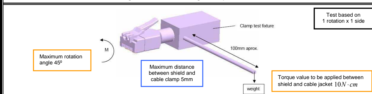
Figure 4: Torsion force test procedure
