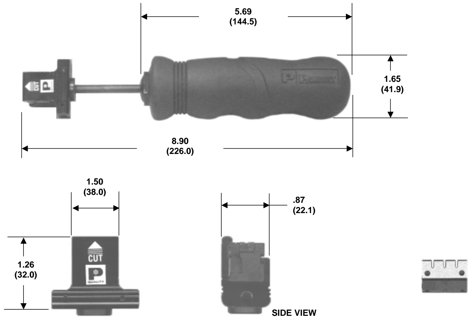
TERMINATION HEAD HOUSING – ALUMINUM GPDTMH
