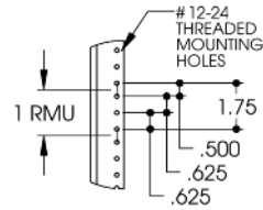
DETAIL A EIA-310-D UNIVERSAL HOLE SPACING
