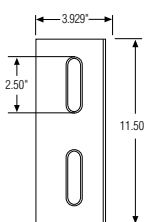
Vertical Channel Divider
