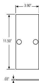
Lateral Channel Divider (rear)
