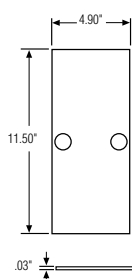
Lateral Channel Divider (front)
