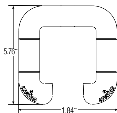
Bend-Radius Compliant Funnel (Use with 4x4 Vertical Slotted Duct only.)
