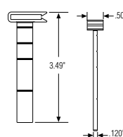
Cable Retainer
