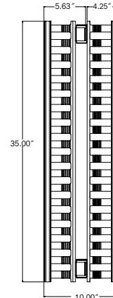
Vertical slotted duct (front and rear)
