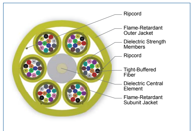
Cross Section of Part Number: 072E81-T3131-24
